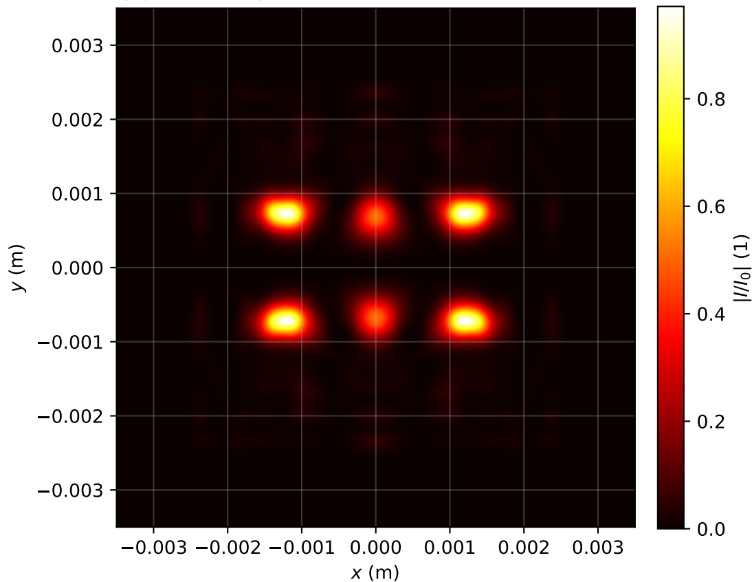
Intensity profile I(x, y, z = 2.786)/I_0 , P_{in}=6.0P_{cr} , artificial time
